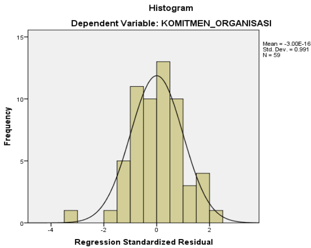
Gambar 1. Histogram
