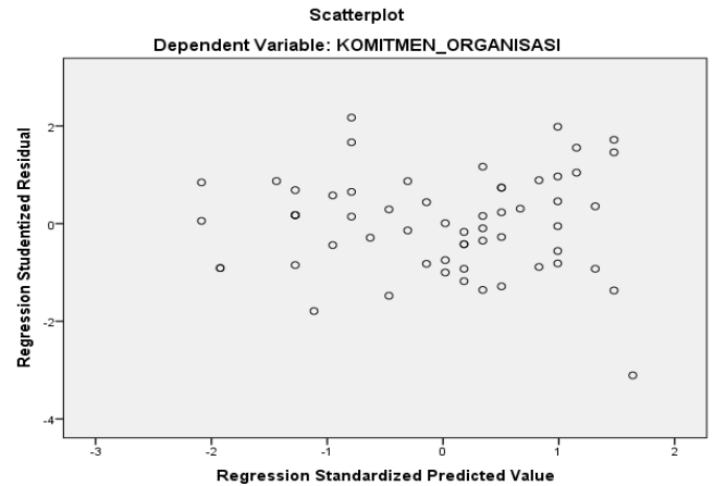
Gambar 2. Scatterplot
